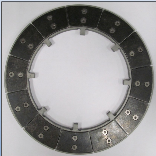
Stator Disk (With wear plates)
